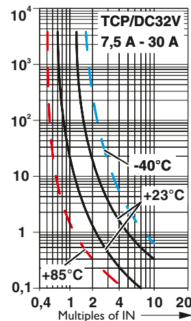
Two key characteristic curves of thermal circuit breakers
