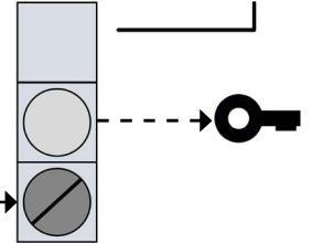
Access key trapped, Personnel (safety) key removed, Access Guard (door) open.
